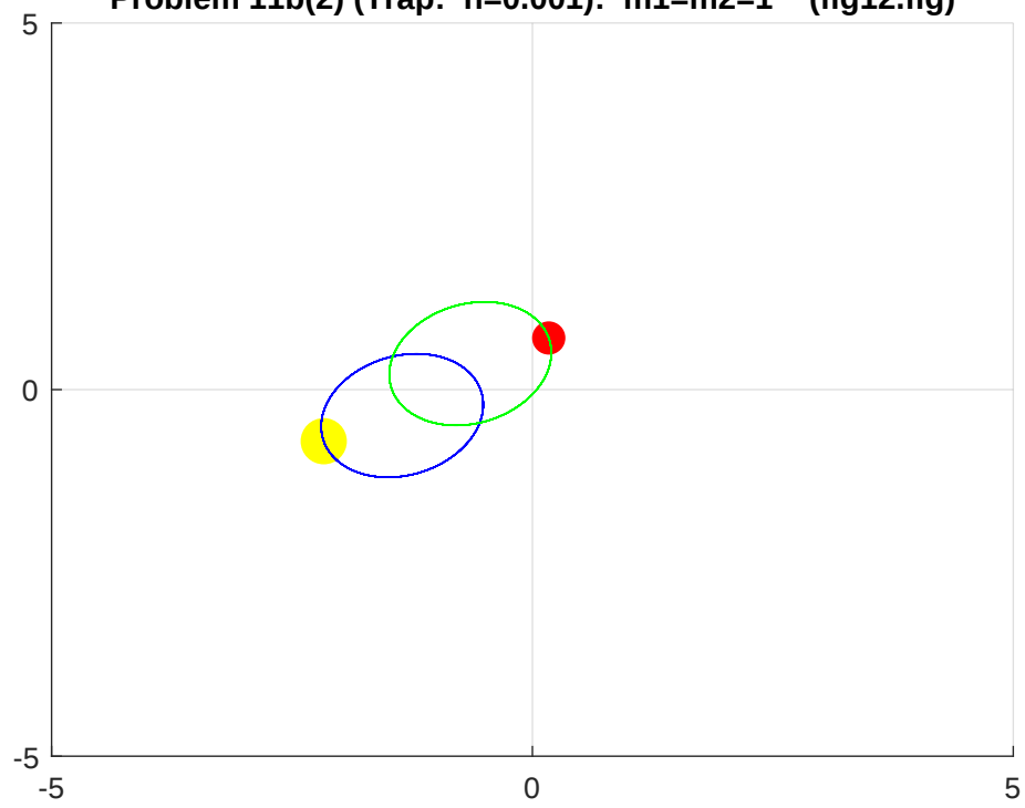
Celestial Mechanics: Two (2) Body Problem Problem 11b(2) (Trap: h=0.001 ): m_1=m_2=1 (fig12.fig)
